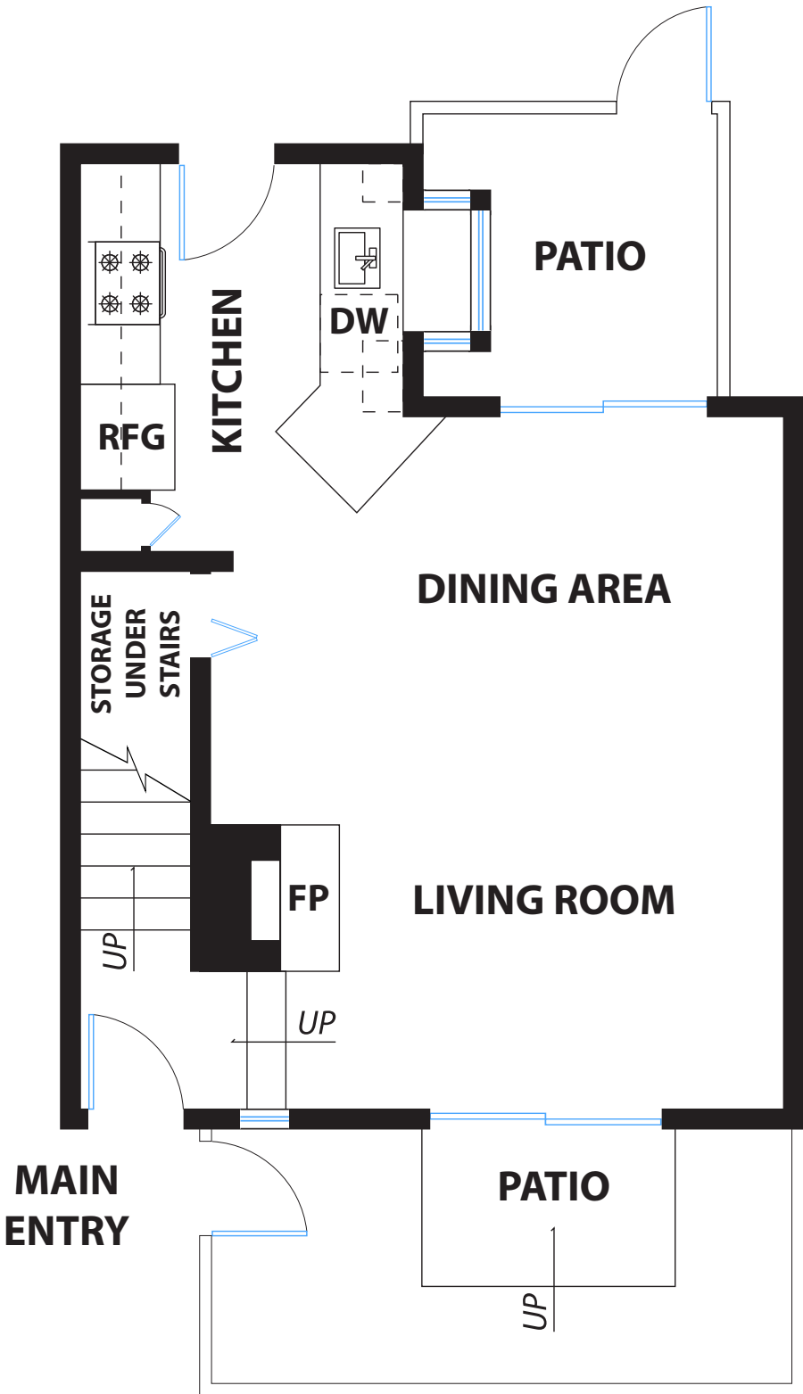
LOWER LEVEL
